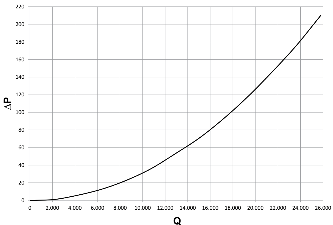
Fig. 23 600 kW plate exchanger flow resistance on primary side and secondary side
