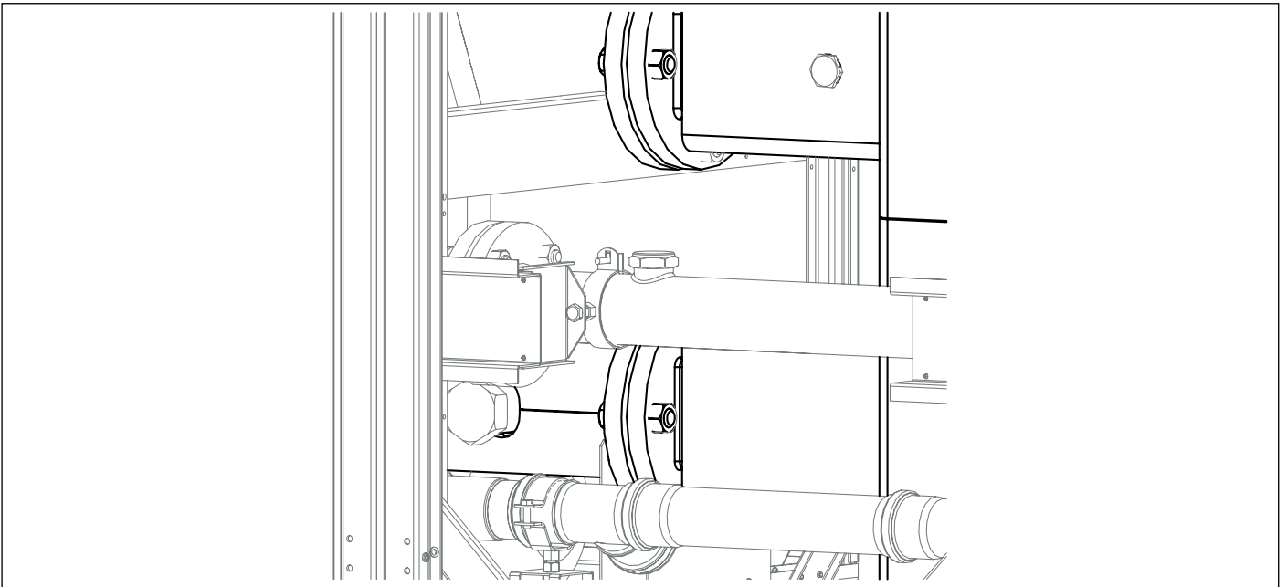
Tighten the screws on the collectors of the intermediate cabinet.
