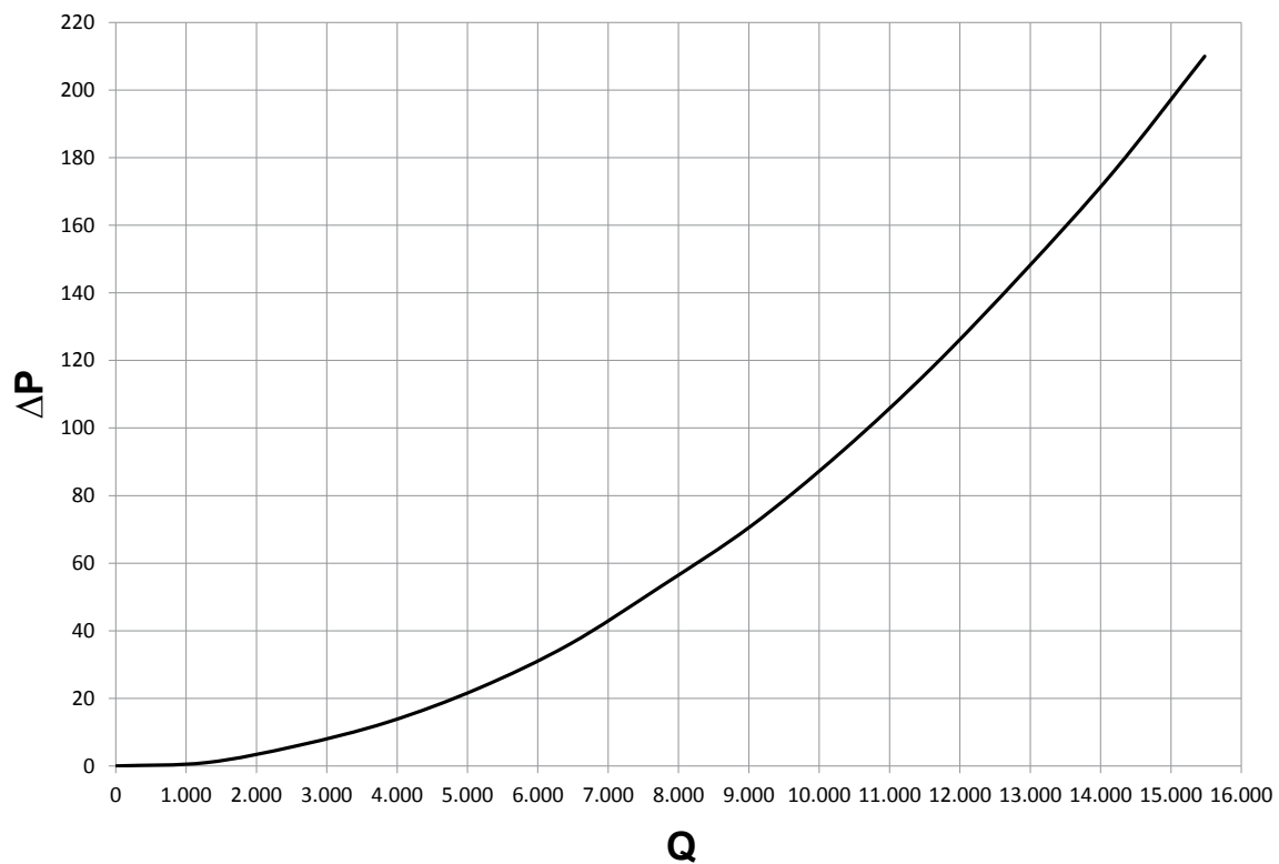
Fig. 20 360 kW plate exchanger flow resistance on primary side and secondary side
