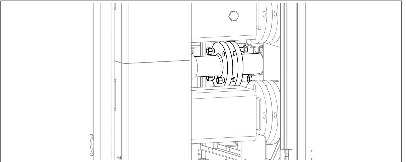
Use the four feet of the cabinet containing the hydraulic separator to align the flow collector, the return collector and the gas pipe to the collectors located inside the adjacent cabinet.
