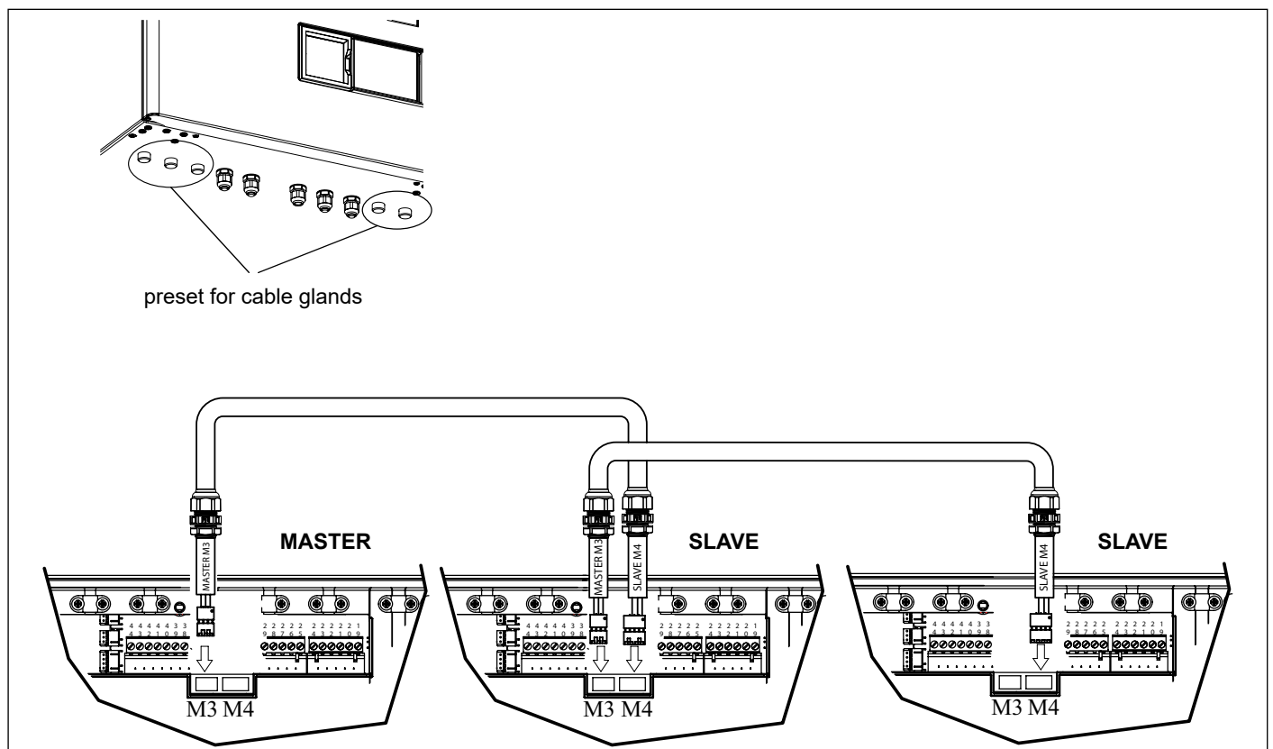
Fig. 32 Cascade connection
