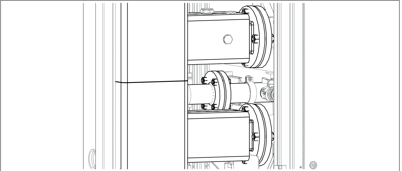
Fasten the flow and return collectors with screws and nuts by placing the gaskets in-between.
