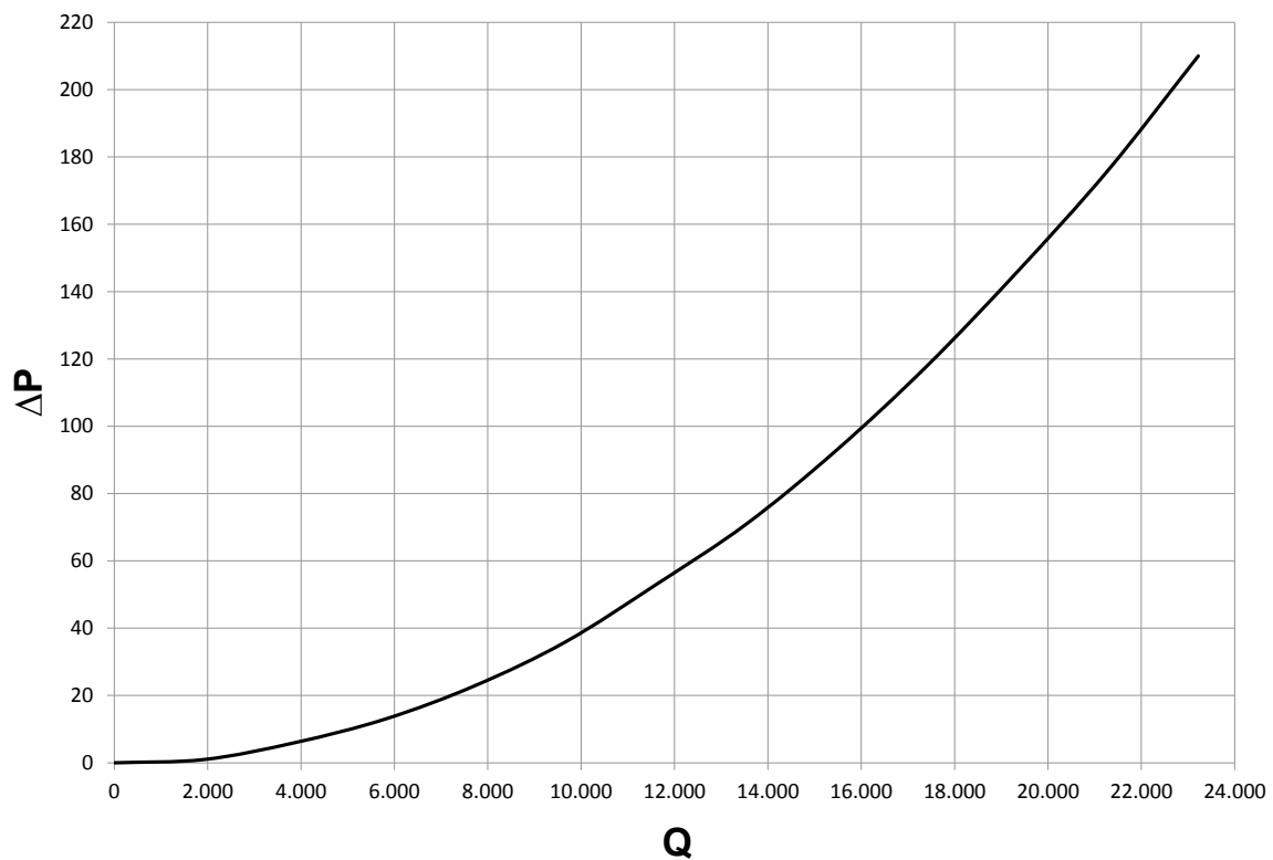
Fig. 22 540 kW plate exchanger flow resistance on primary side and secondary side
