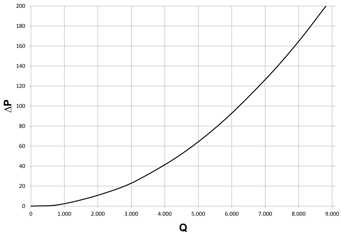
Fig. 18 205 kW plate exchanger flow resistance on primary side and secondary side
