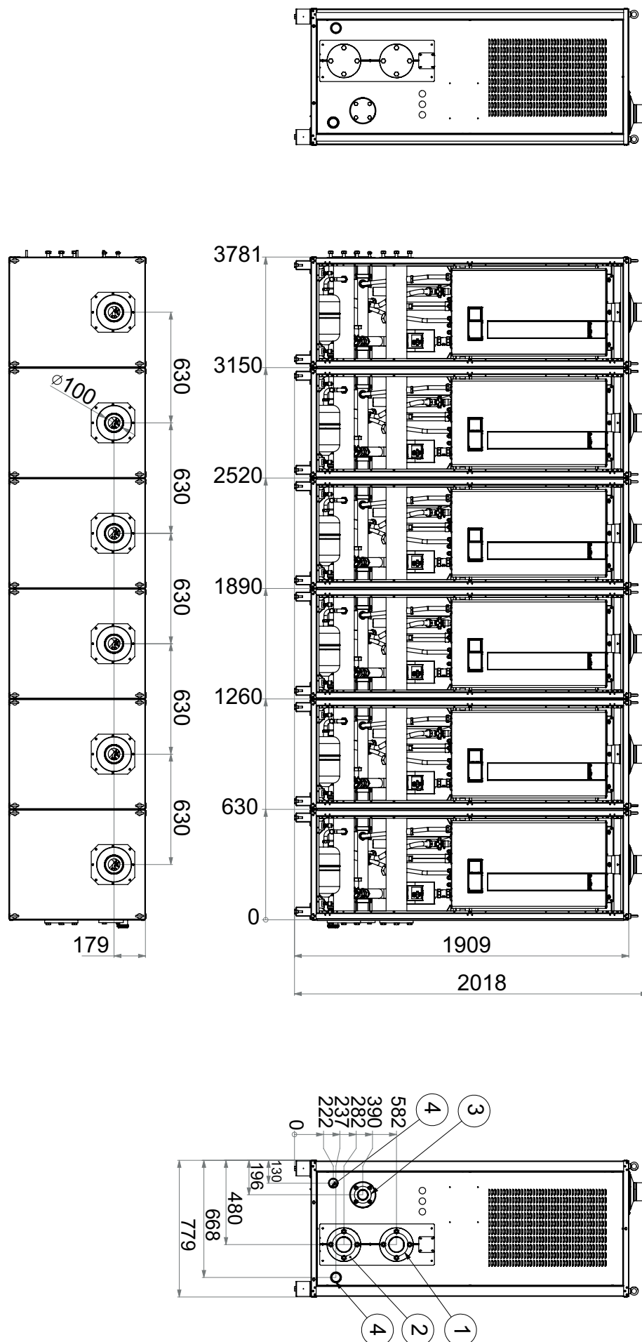
Fig. 3 Combination of left 120-150 direct collectors in cabinet
