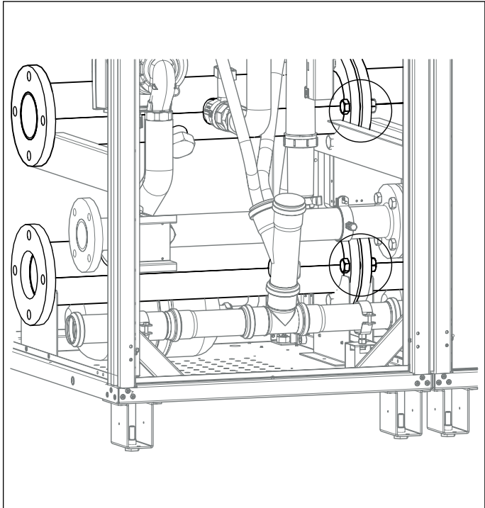
Fasten the flow and return collectors with screws and nuts by placing the gaskets in-between.
