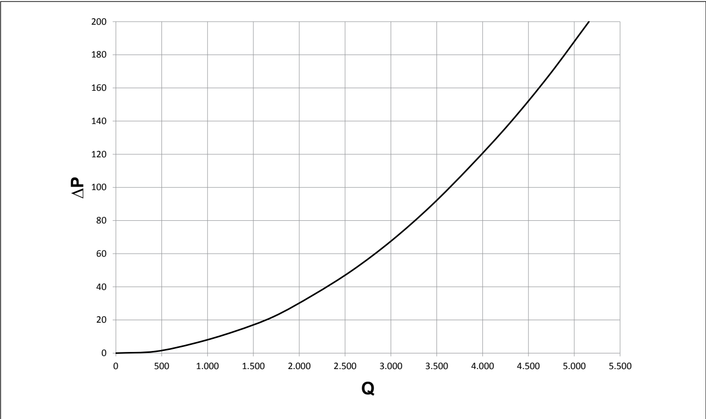
Fig. 17 120 kW plate exchanger flow resistance on primary side and secondary side
