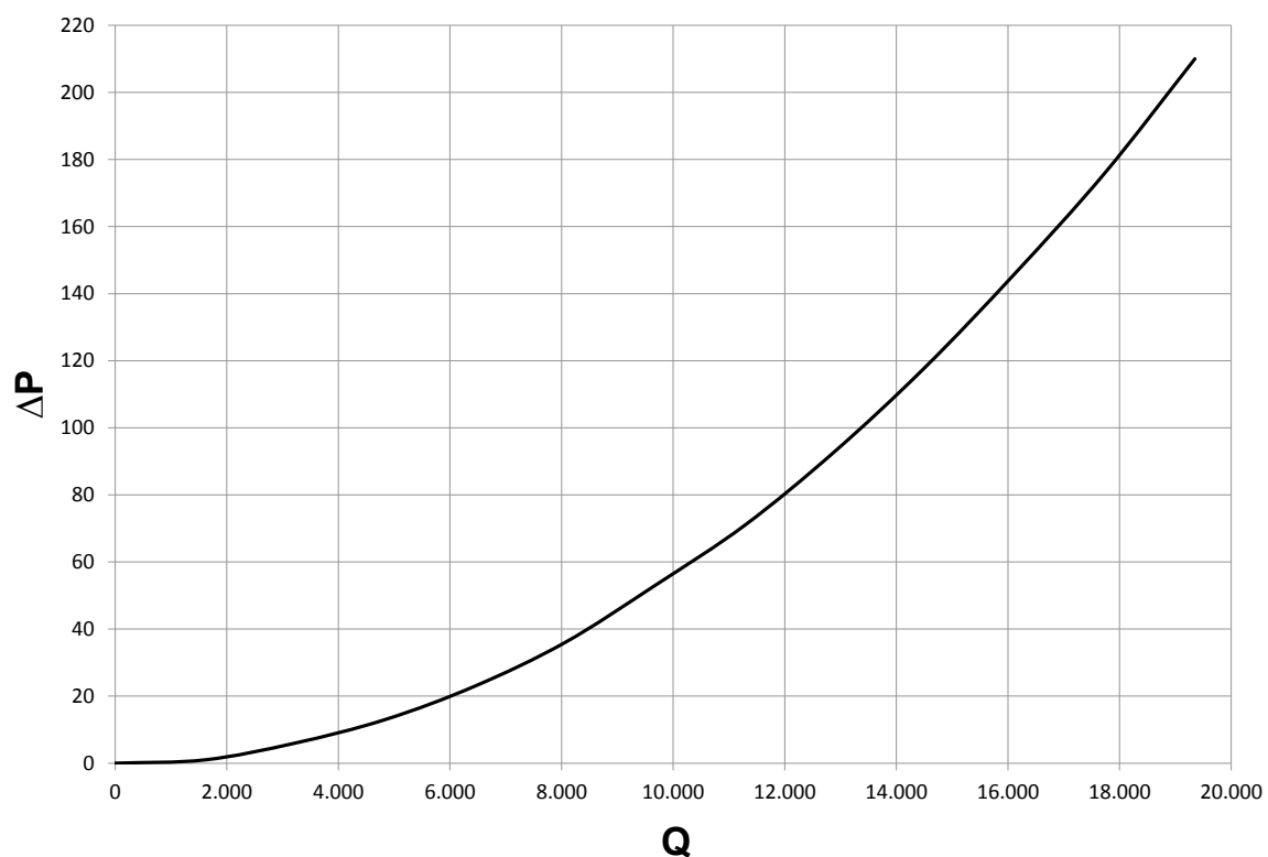
Fig. 21 450 kW plate exchanger flow resistance on primary side and secondary side
