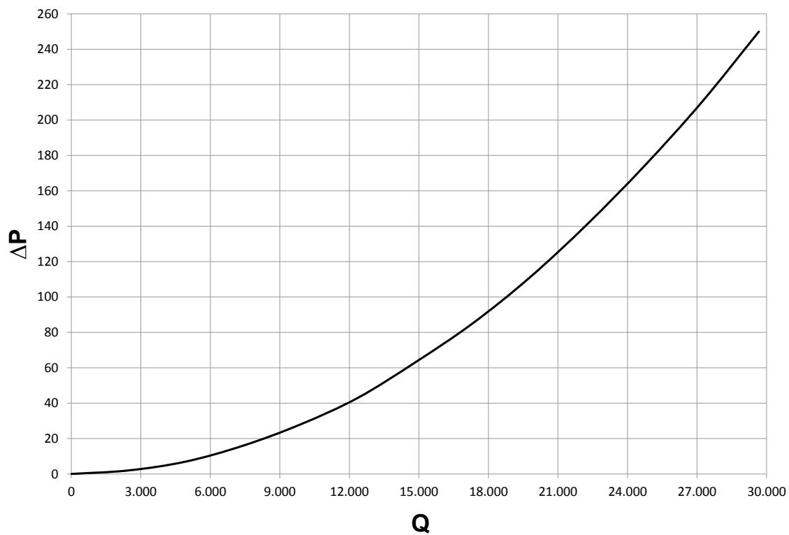
Fig. 24 690 kW plate exchanger flow resistance on primary side and secondary side
