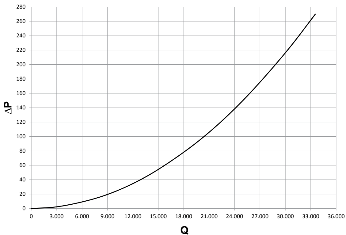
Fig. 25 780 kW plate exchanger flow resistance on primary side and secondary side
