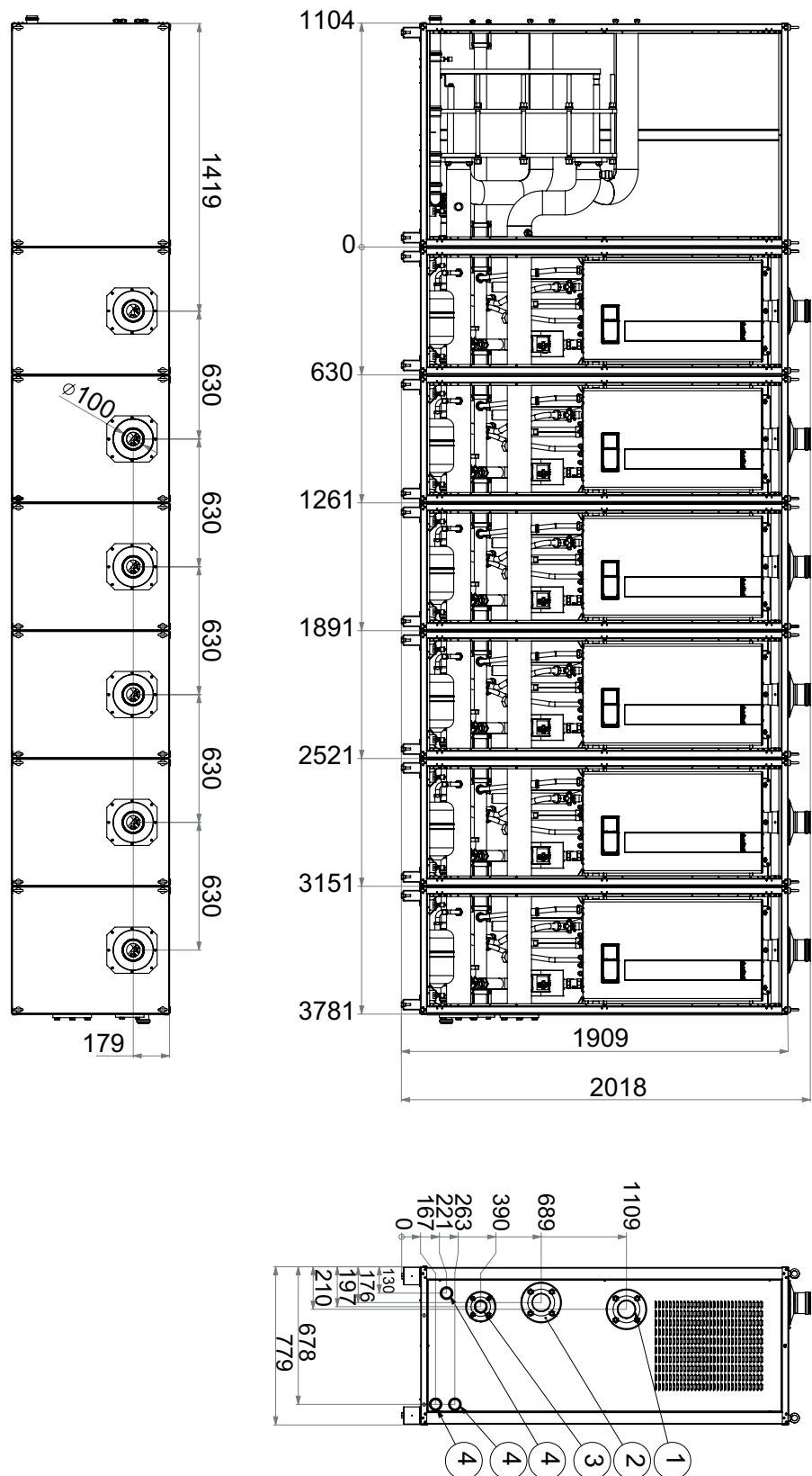
Fig. 14 Combination of left 120-150 plate exchanger in cabinet
