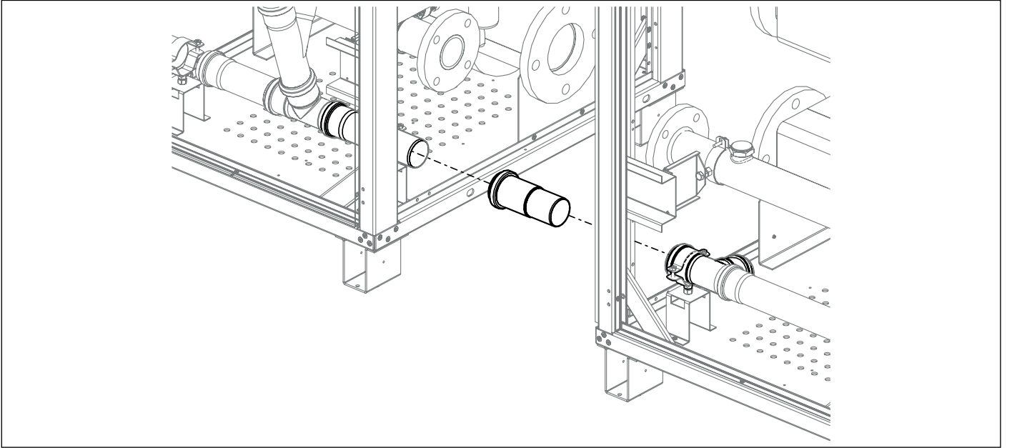
Assemble the supplied pipe on the condensate drain as shown in the image.
