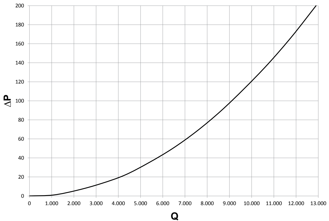
Fig. 19 300 kW plate exchanger flow resistance on primary side and secondary side
