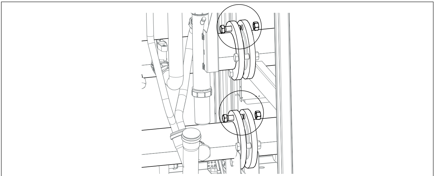
Fasten the flow and return collectors with screws and nuts by placing the gaskets in-between.
