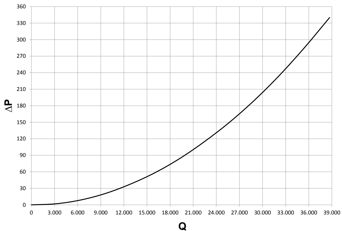
Fig. 26 900 kW plate exchanger flow resistance on primary side and secondary side
