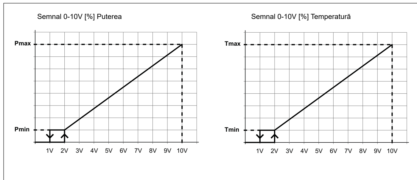
Fig. 23 Semnal 0-10VDC
