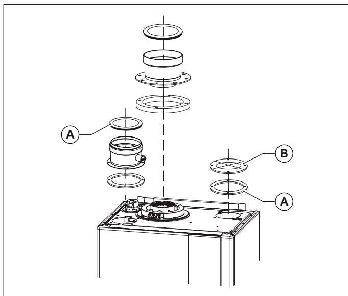
Fig. 18 Conducte coaxiale tip C43 – C53 – C83
