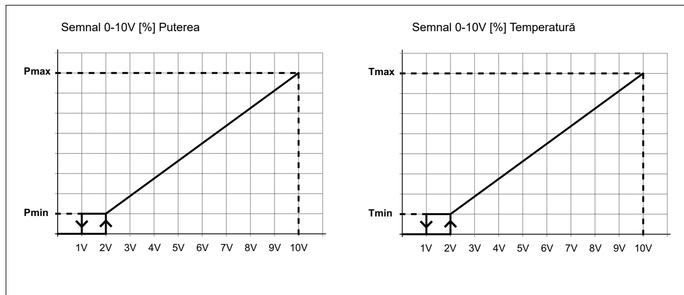
Fig. 23 Semnal 0-10VDC
