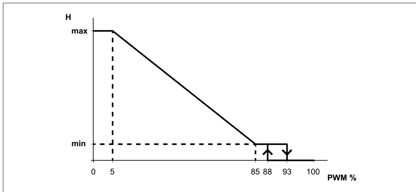
Fig. 25 Semnal PWM
