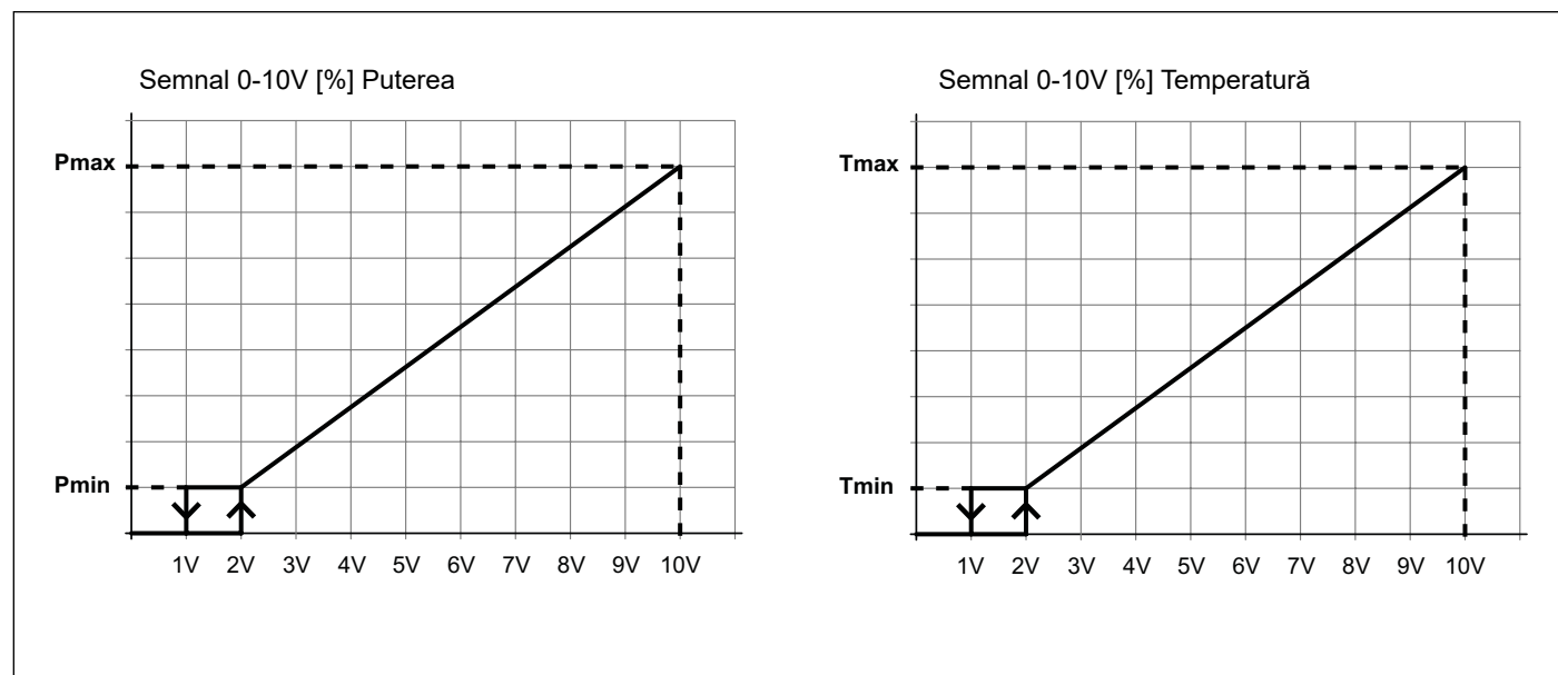
Fig. 20 Semnal 0-10VDC
