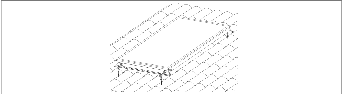
fig. 10 - Installation on sloping roof through tile or pantile
