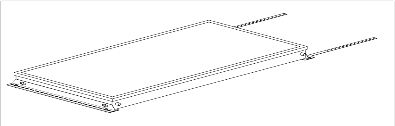
fig. 6 - Collector roof installation
