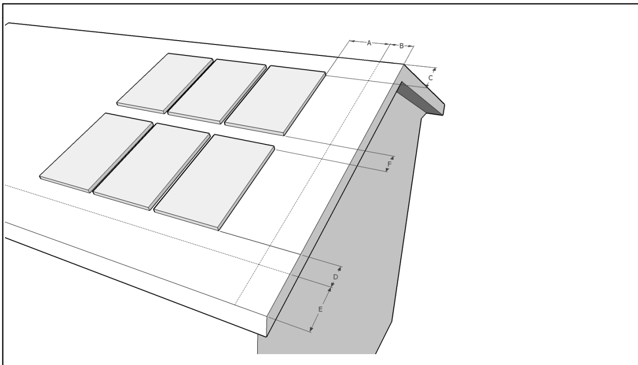
fig. 4 - Installation distances
